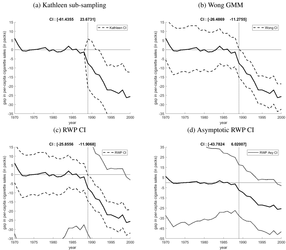
Figure 2: Analytical confidence intervals
