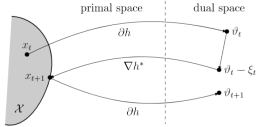
Figure 1: Iterates of UMD
